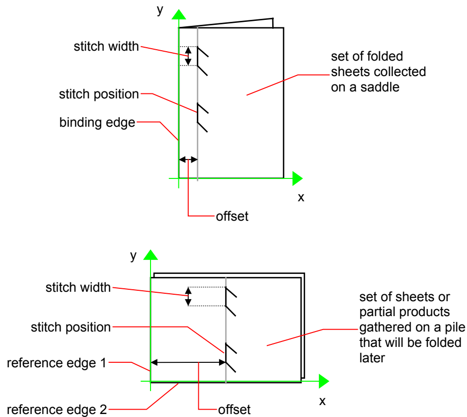
Figure 7.18 Parameters and coordinate system used for stitching
