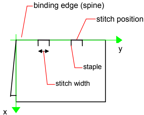
Figure 7.16 Parameters and coordinate system used for saddle stitching
