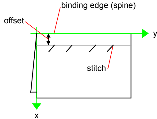
Figure 7.17 Parameters and coordinate system used for side sewing
