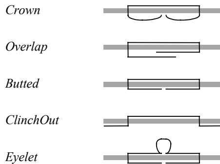
Figure 7.15 Staple shapes
