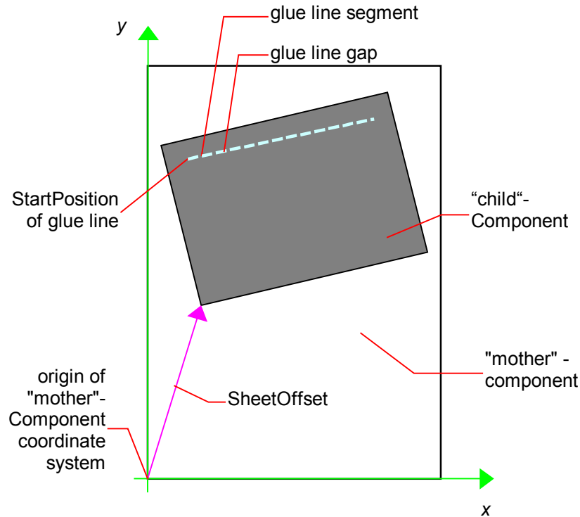
Figure 7.14 Parameters and coordinate system used for inserting
